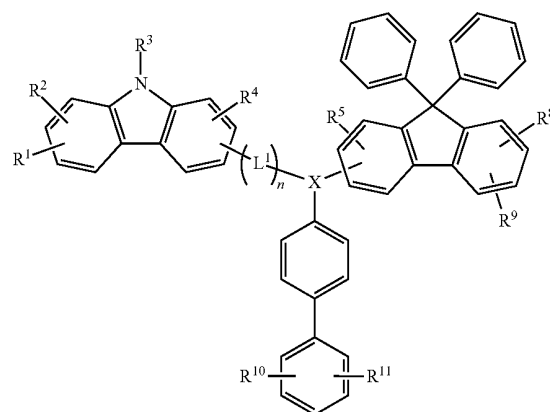
[Chemical Formula 6]
