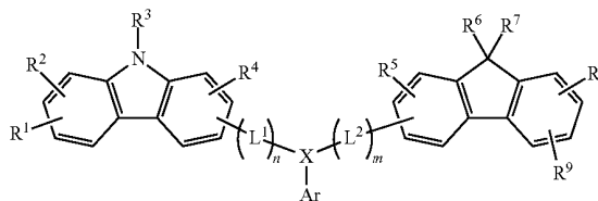
[Chemical Formula 1]
