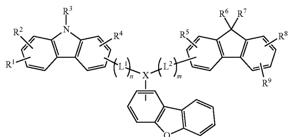
[Chemical Formula 3]
