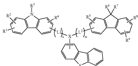
[Chemical Formula 4]
